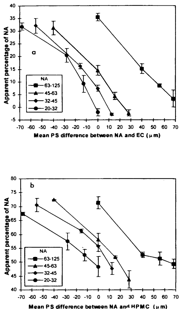
Fig. 3. Apparent percentage of niflumic acid in 50/50 v/v binary mixes of niflumic acid and ethyl cellulose (a) or hydroxypropyl methylcellulose (b) compacted at 44.0 kN as a function of the difference between their mean particle sizes (mean PS). When error bars are not visible, they are included within the size of the symbols.
