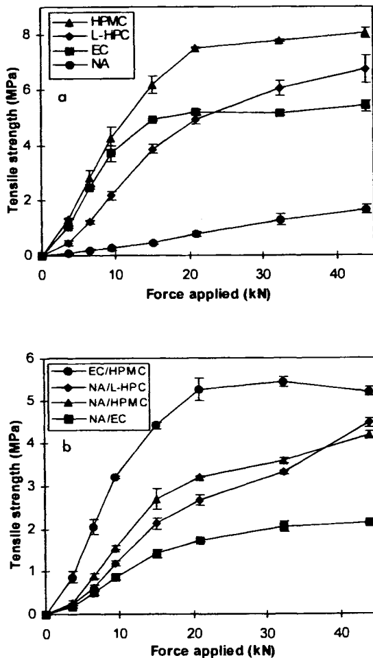
Fig. 1. Tensile strengths of compacts of pure NA, EC, HPMC and L-HPC (a) and of their 50/50 v/v mixes (b) obtained at different compression forces. When error bars are not visible, they are included within the size of the symbols.
