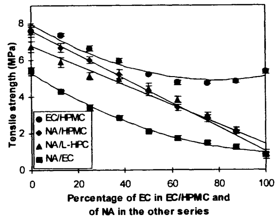
Fig. 2. Tensile strength of compacts obtained at 44.0 kN containing different proportions of ethyl cellulose or niflumic acid in the EC/HPMC ( y = 0.0005x^2 - 0.0780x + 8.0088 ), NA/HPMC ( y = -0.0658x + 7.6190 ), NA/L-HPC ( y = -0.0537x + 6.8000 ) and NA/EC ( y = 0.0004x^2 - 0.0807x + 5.3093 ) series. When error bars are not visible, they are included within the size of the symbols.
