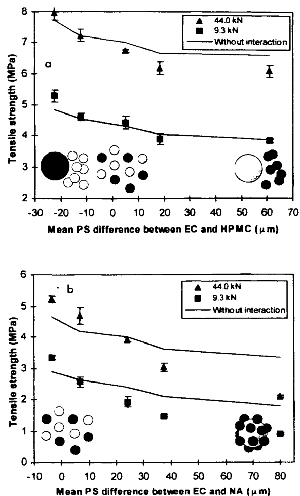
Fig. 6. Experimental tensile strength of HPMC/freeze-milled EC (a) and NA/freeze-milled EC (b) tablets obtained at two compression forces (9.3 and 44.0 kN) compared to the expected value without interaction (in continued line). When error bars are not visible, they are included within the size of the symbols.
