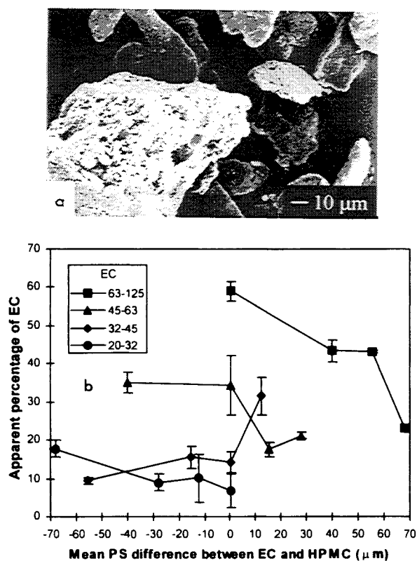
Fig. 5. SEM pictures of the 20–32 μm fraction of HPMC blended with the 63–125 μm fraction of ethyl cellulose (a) and apparent percentage of ethyl cellulose in 50/50 v/v binary mixes of ethyl cellulose and hydroxypropyl methylcellulose compacted at 44.0 kN as a function of the difference between their mean particle sizes (b). When error bars are not visible, they are included within the size of the symbols.
